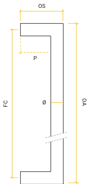
MITRED PULL HANDLE
